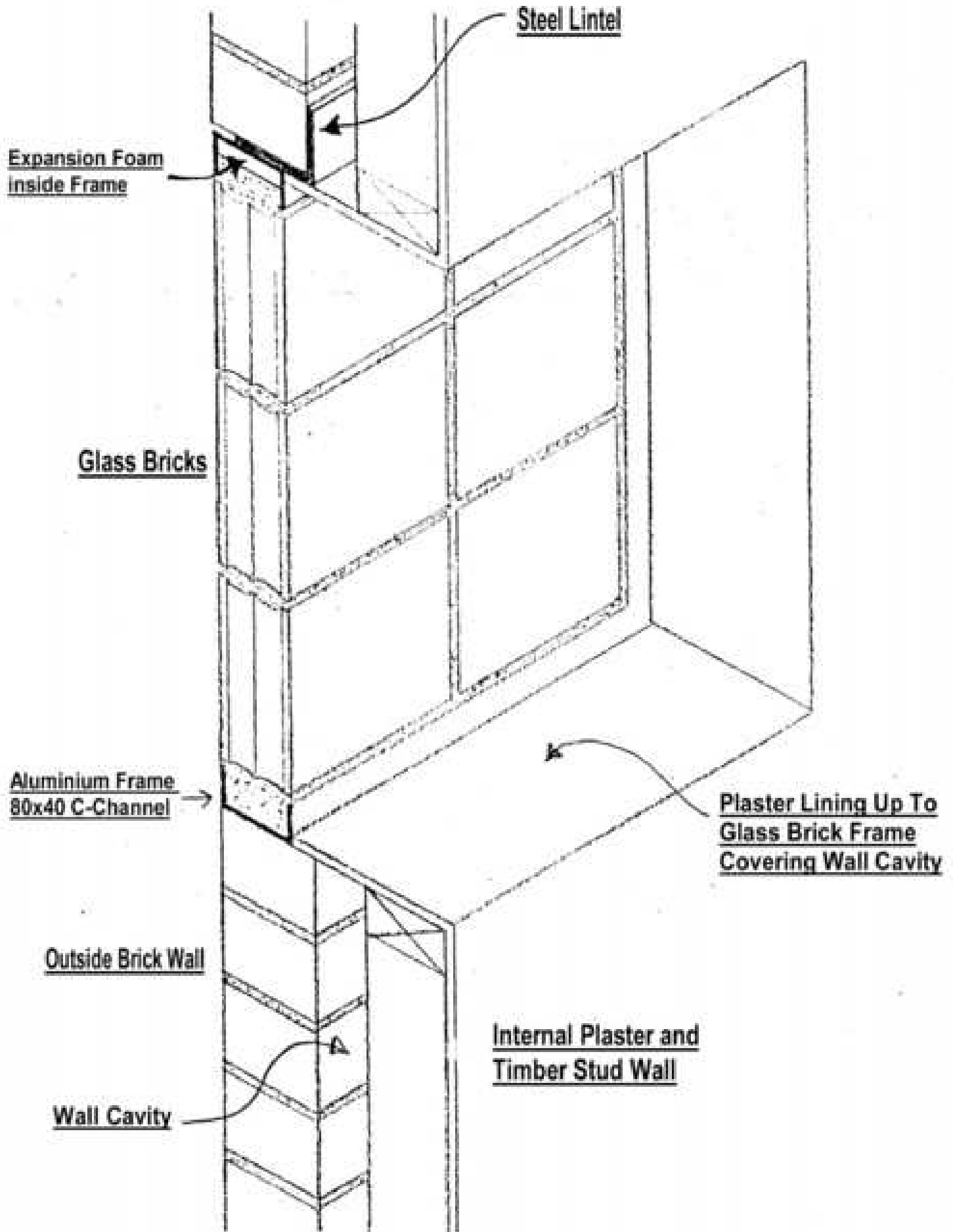
SECTION THROUGH BRICK VENEER WALL
